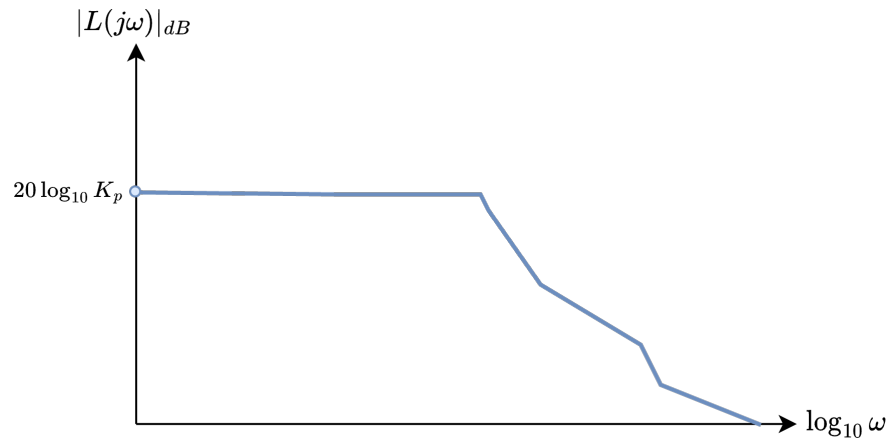
Figure 10.11 : Frequency response magnitude of loop transfer function, showing determination of position error constant, K_p .
