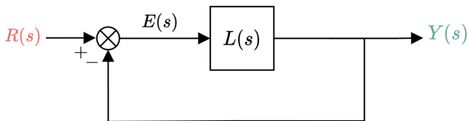
Figure 10.1: Block diagram of system in unity feedback.
