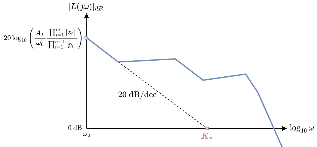
Figure 10.12 : Frequency response magnitude of loop transfer function, showing determination of velocity error constant, K_v .
