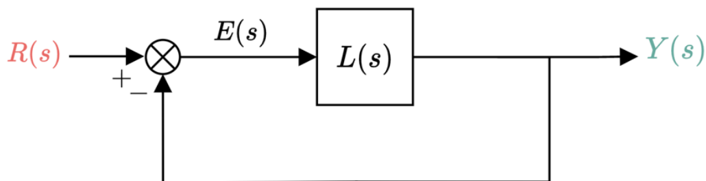
Figure 10.10 : Block diagram of closed-loop system.
