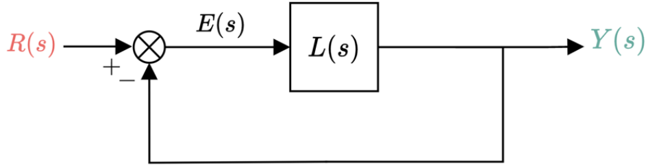
Figure 10.5: System in unity feedback.
