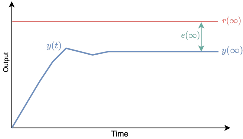
Figure 10.6: Finite steady-state error, e(\infty) , from step-like reference signal.
