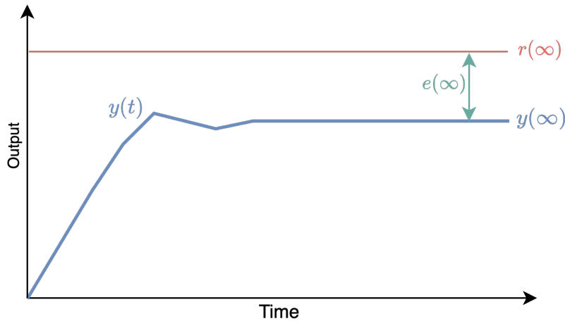
Figure 10.2: Finite steady-state error from step-like reference signal.
