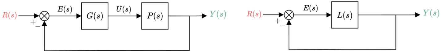
Figure 10.8 : Equivalent closed-loop systems.
