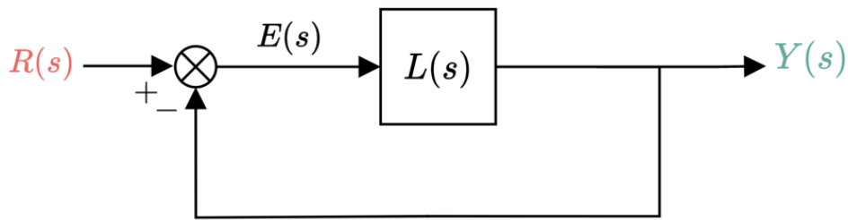
Figure 10.4: System in unity feedback.
