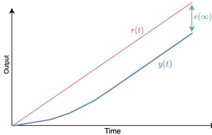
Figure 10.3: Finite steady-state error from ramp-like reference signal.
