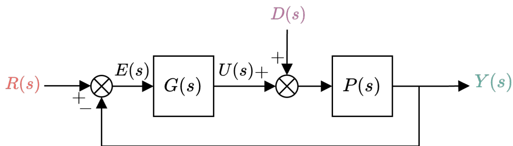
Figure 10.9 : Block diagram of closed-loop system with plant input disturbance.
