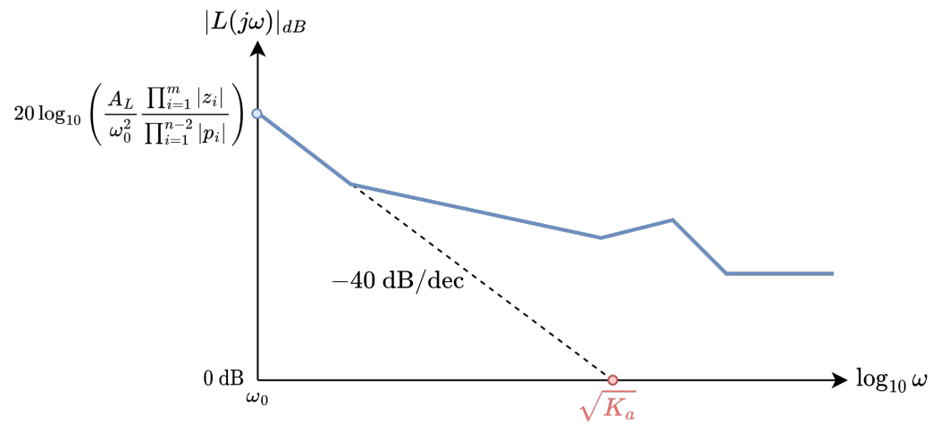
Figure 10.13 : Frequency response magnitude of loop transfer function, showing determination of acceleration error constant, K_a .
